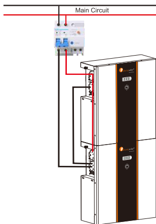
Step 2: The schematic diagram of the parallel connection of two battery packs is shown in Figure 2.
